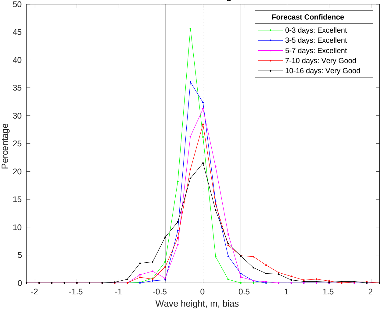
NDBC 42036 vs GFS Waves Bias Histogram: 20-Jul-2025
