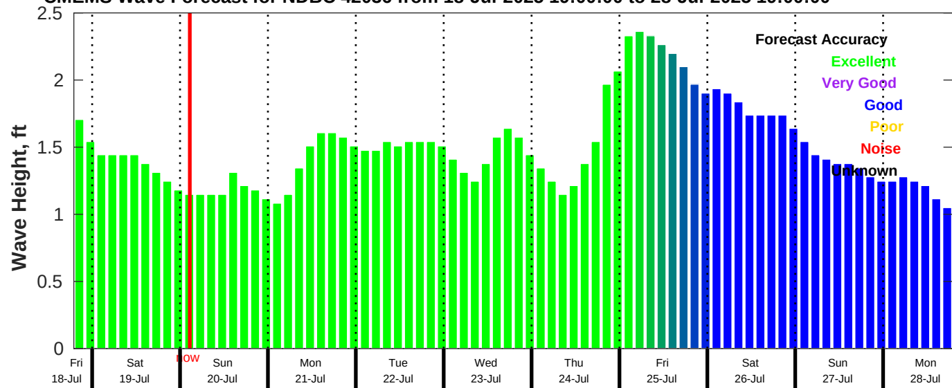
CMEMS Wave Forecast for NDBC 42036 from 18-Jul-2025 19:00:00 to 28-Jul-2025 19:00:00
