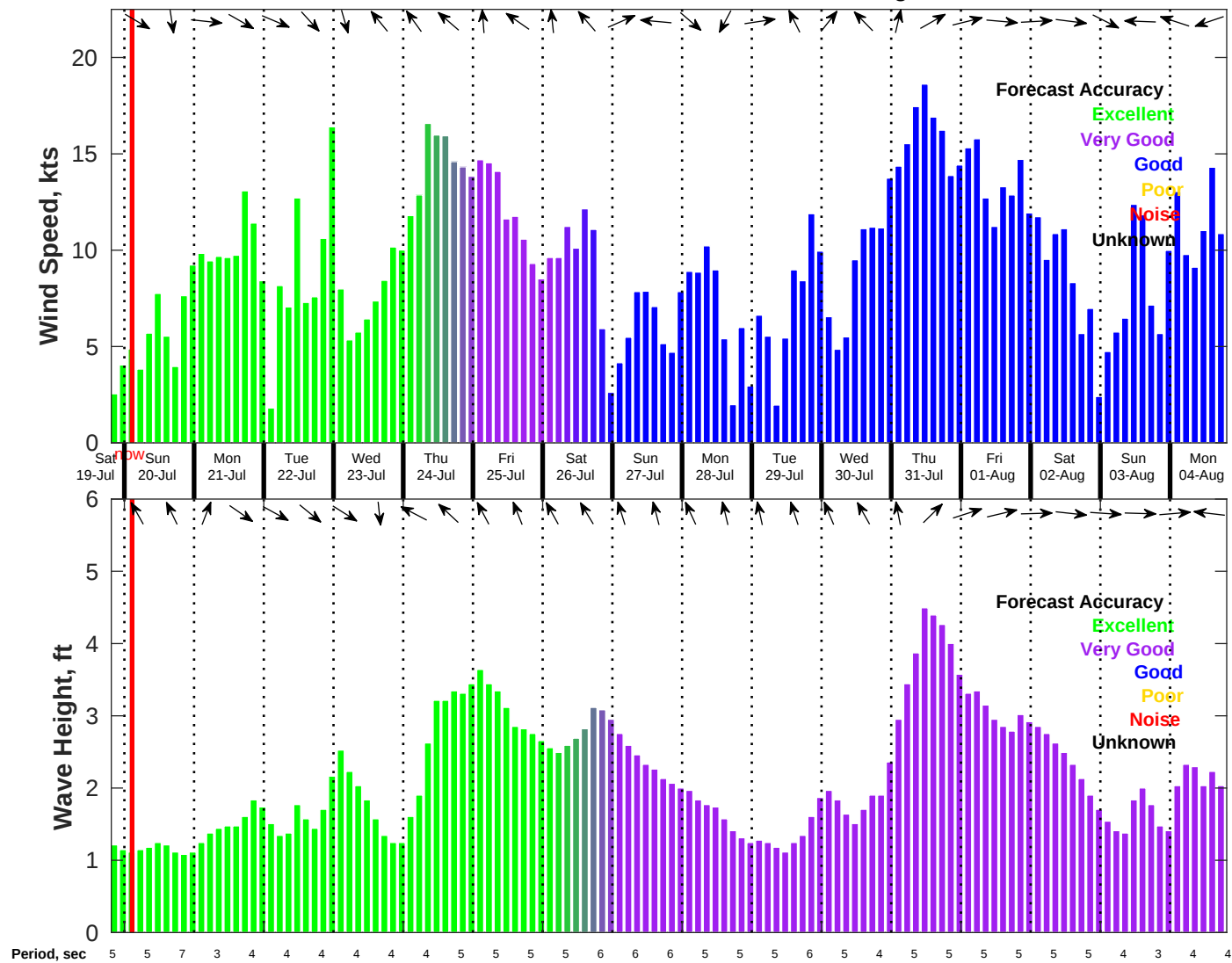
Wind & Wave Forecast for NDBC 42036 from 19-Jul-2025 19:00:00 to 04-Aug-2025 19:00:00
