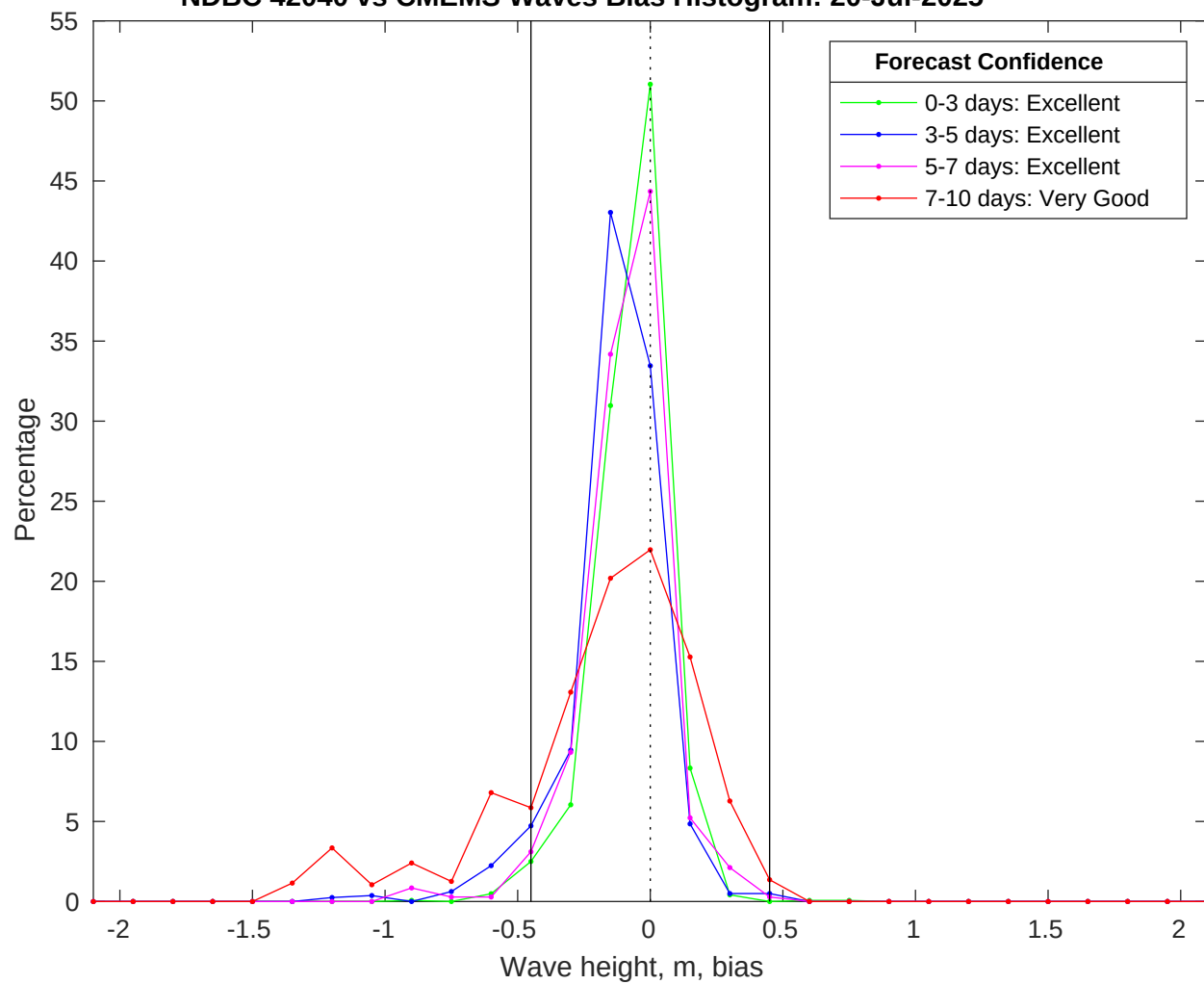
NDBC 42040 vs CMEMS Waves Bias Histogram: 20-Jul-2025
