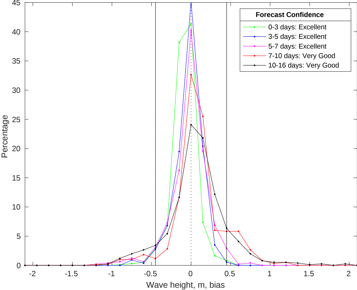
NDBC 42040 vs GFS Waves Bias Histogram: 20-Jul-2025
