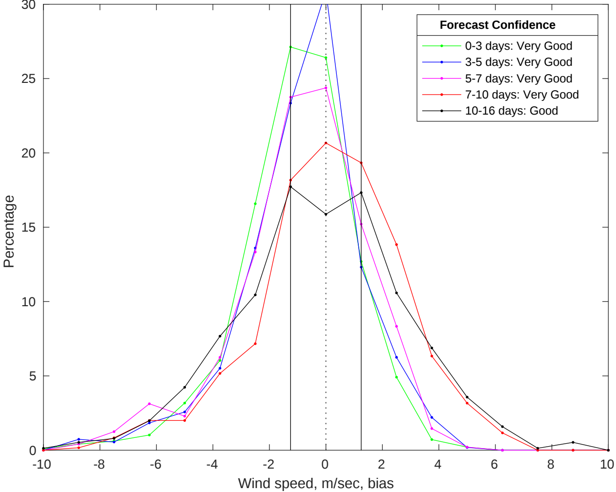
NDBC 42040 vs GFS Winds Bias Histogram: 20-Jul-2025
