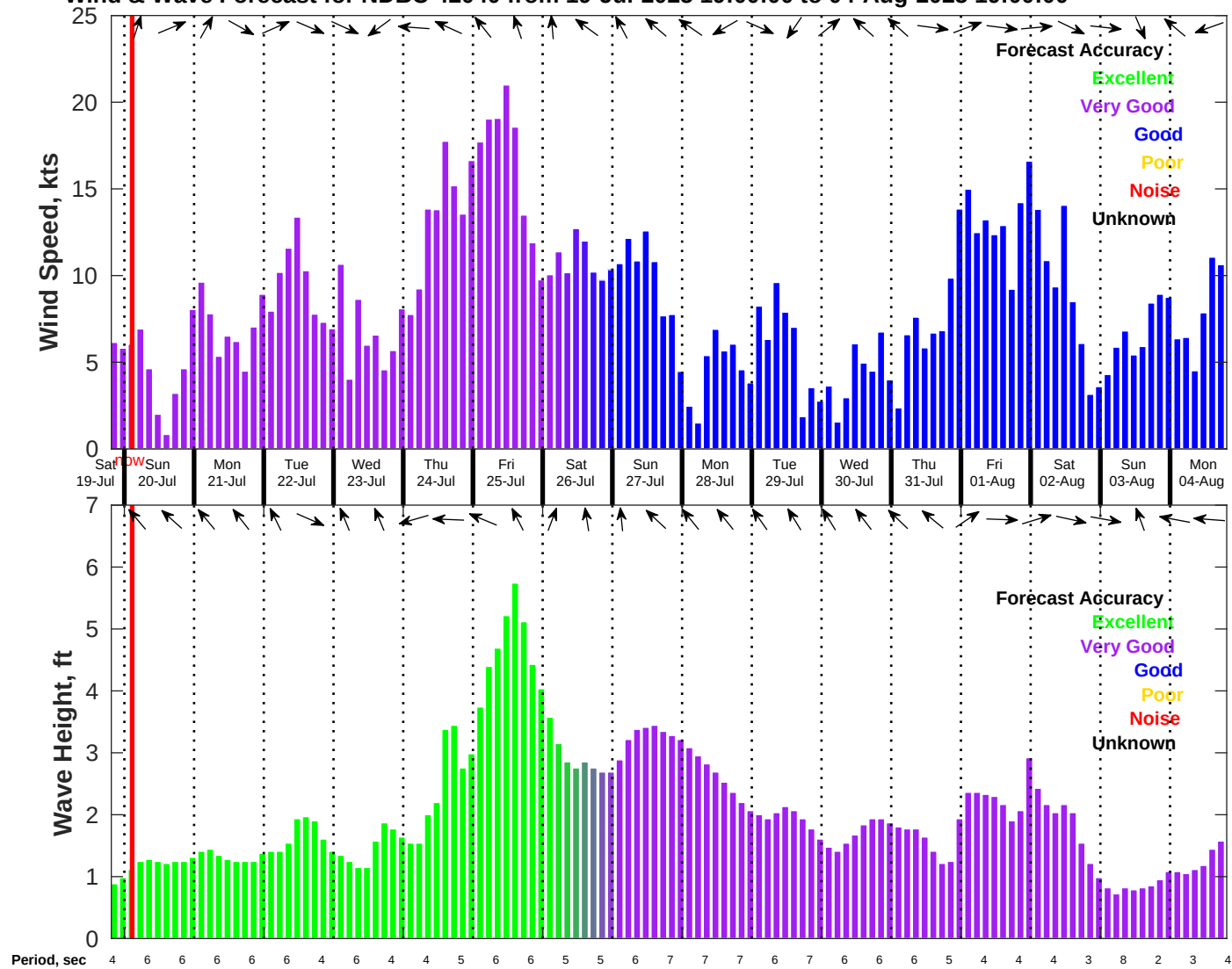
Wind & Wave Forecast for NDBC 42040 from 19-Jul-2025 19:00:00 to 04-Aug-2025 19:00:00
