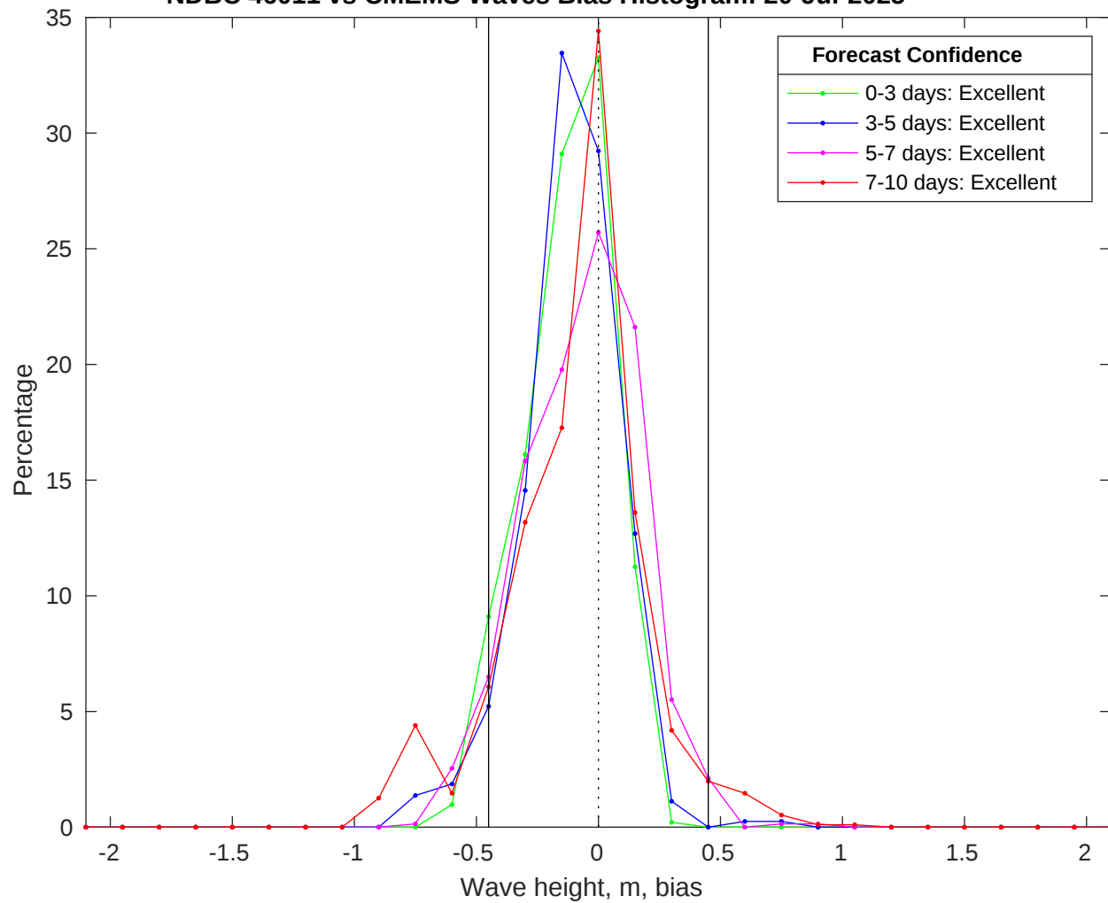
NDBC 46011 vs CMEMS Waves Bias Histogram: 20-Jul-2025
