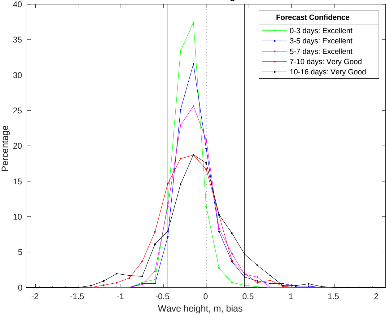
NDBC 46011 vs GFS Waves Bias Histogram: 20-Jul-2025
