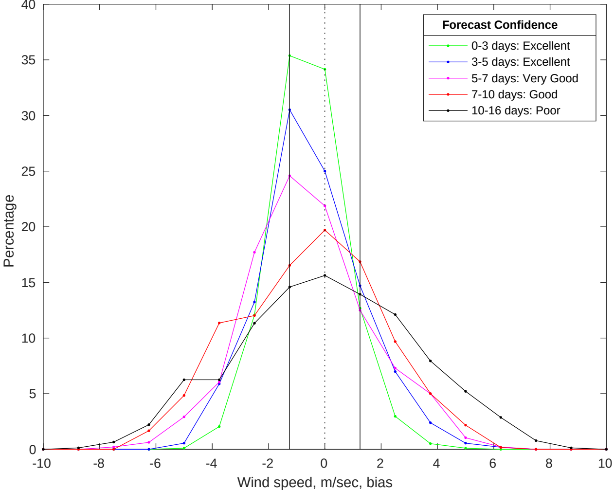
NDBC 46011 vs GFS Winds Bias Histogram: 20-Jul-2025
