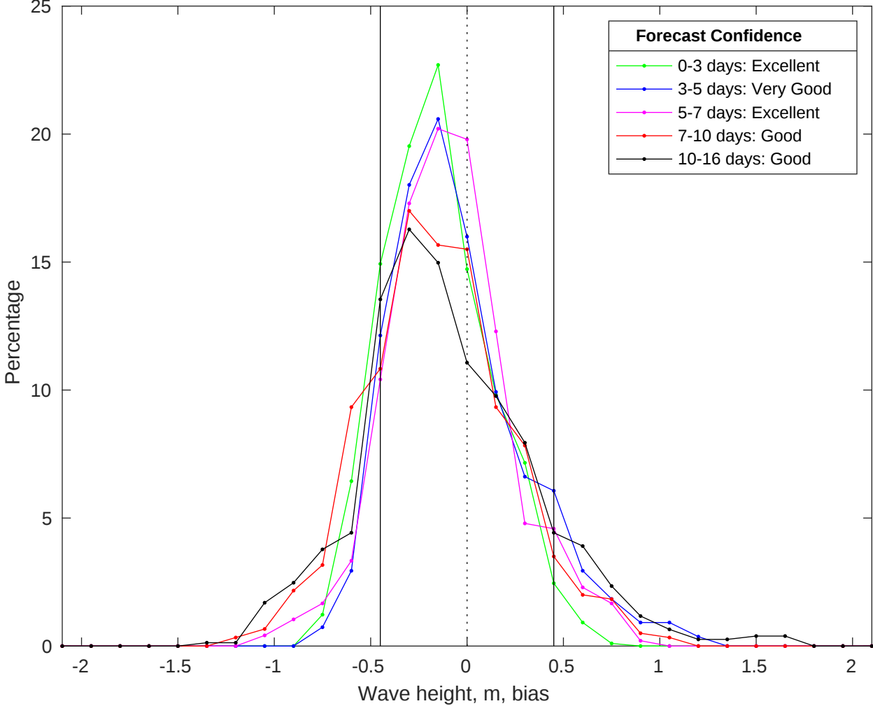
NDBC 46028 vs GFS Waves Bias Histogram: 20-Jul-2025
