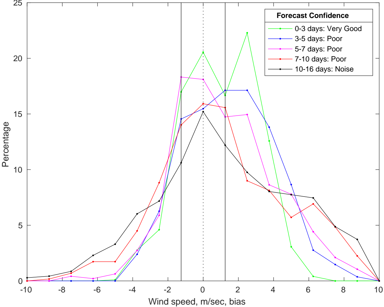
NDBC 46028 vs GFS Winds Bias Histogram: 20-Jul-2025
