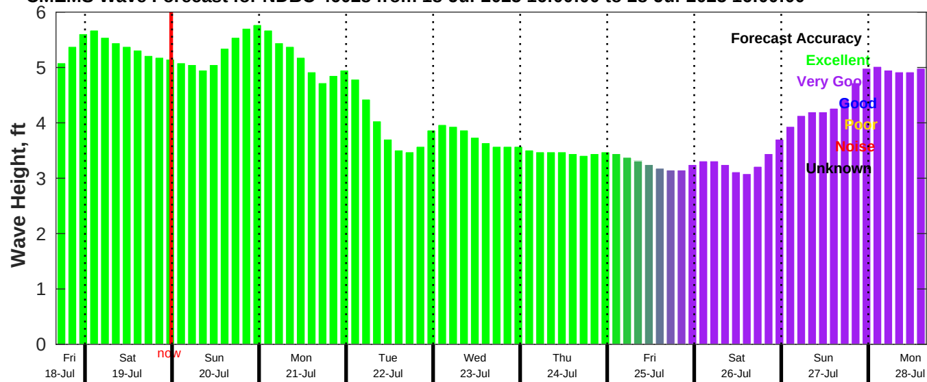
CMEMS Wave Forecast for NDBC 46028 from 18-Jul-2025 16:00:00 to 28-Jul-2025 16:00:00
