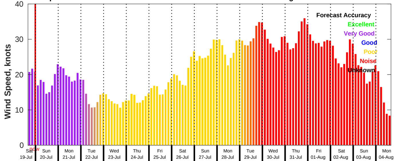
GFS Wind Speed Forecast for NDBC 46028 from 19-Jul-2025 16:00:00 to 04-Aug-2025 16:00:00
