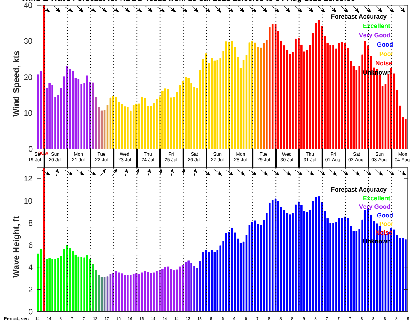
Wind & Wave Forecast for NDBC 46028 from 19-Jul-2025 16:00:00 to 04-Aug-2025 16:00:00
