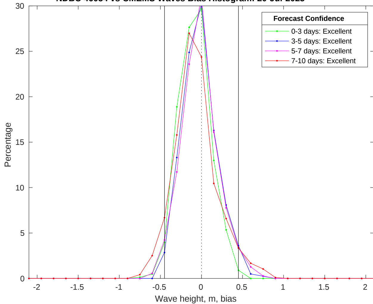
NDBC 46054 vs CMEMS Waves Bias Histogram: 20-Jul-2025
