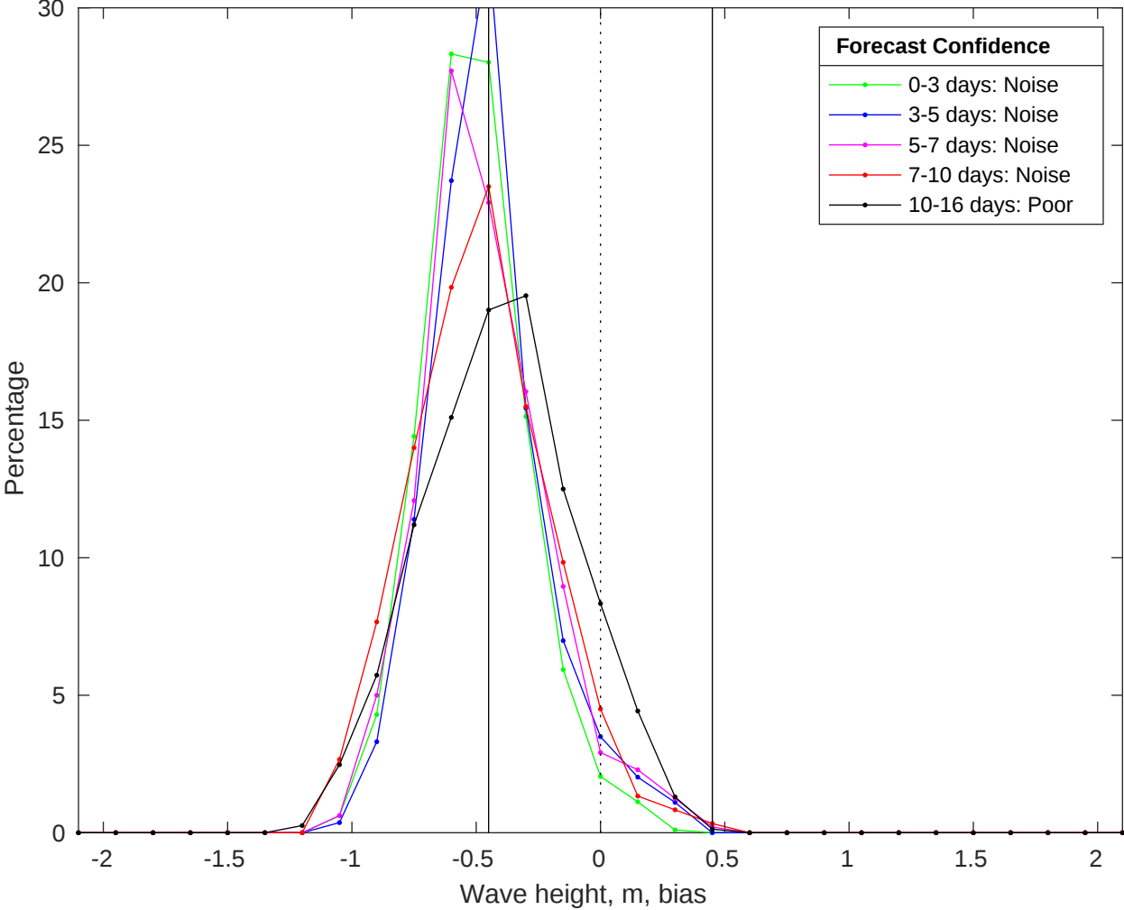
NDBC 46054 vs GFS Waves Bias Histogram: 20-Jul-2025
