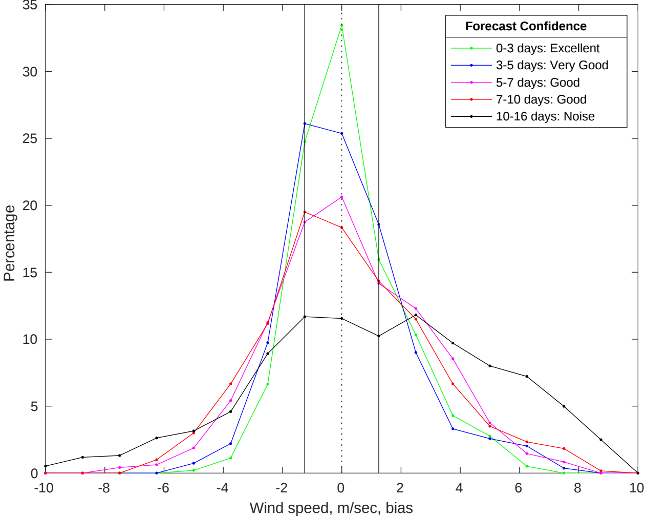
NDBC 46054 vs GFS Winds Bias Histogram: 20-Jul-2025
