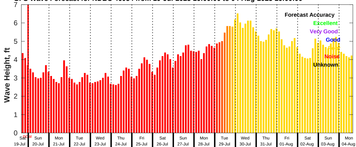
GFS Wave Forecast for NDBC 46054 from 19-Jul-2025 16:00:00 to 04-Aug-2025 16:00:00
