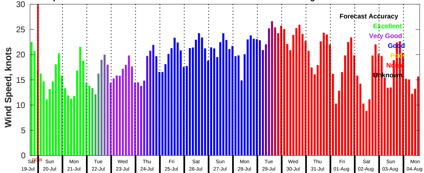
GFS Wind Speed Forecast for NDBC 46054 from 19-Jul-2025 16:00:00 to 04-Aug-2025 16:00:00
