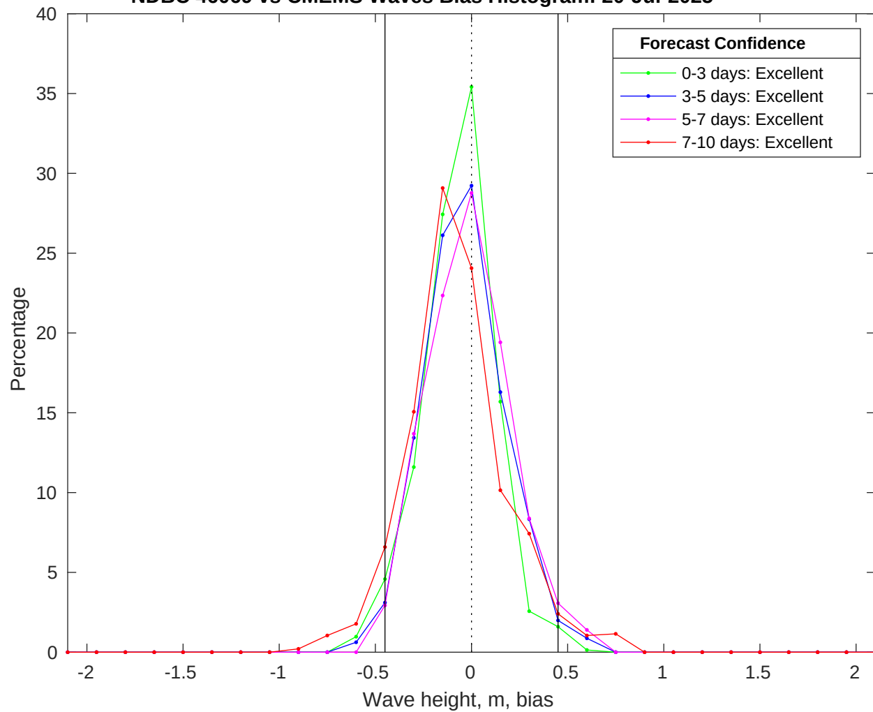
NDBC 46069 vs CMEMS Waves Bias Histogram: 20-Jul-2025
