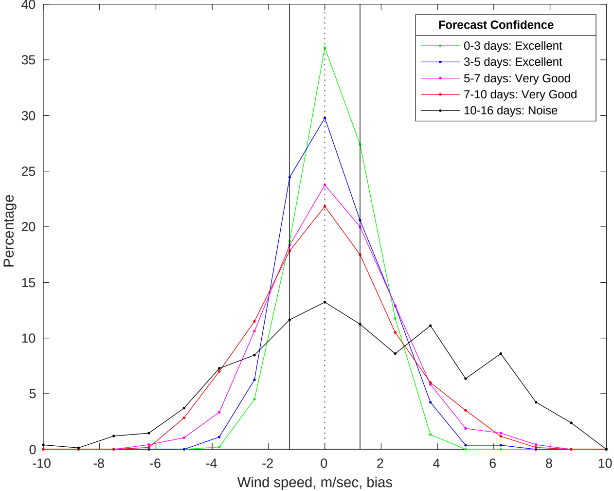
NDBC 46069 vs GFS Winds Bias Histogram: 20-Jul-2025
