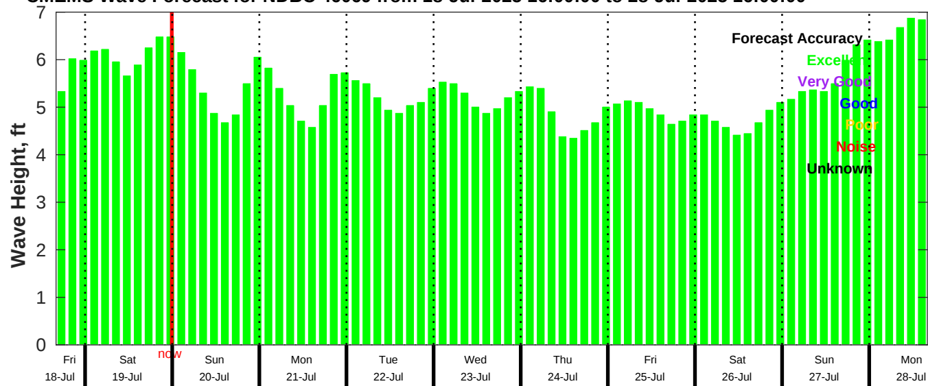
CMEMS Wave Forecast for NDBC 46069 from 18-Jul-2025 16:00:00 to 28-Jul-2025 16:00:00
