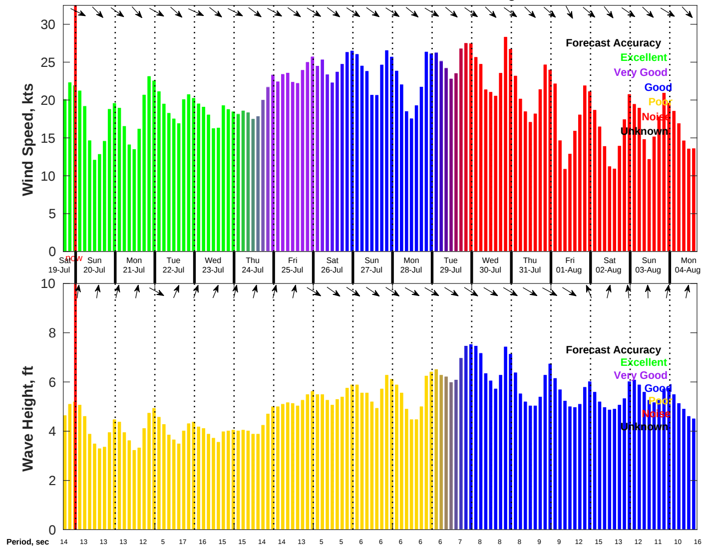
Wind & Wave Forecast for NDBC 46069 from 19-Jul-2025 16:00:00 to 04-Aug-2025 16:00:00
