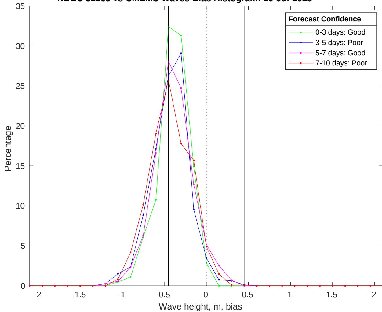
NDBC 51209 vs CMEMS Waves Bias Histogram: 20-Jul-2025
