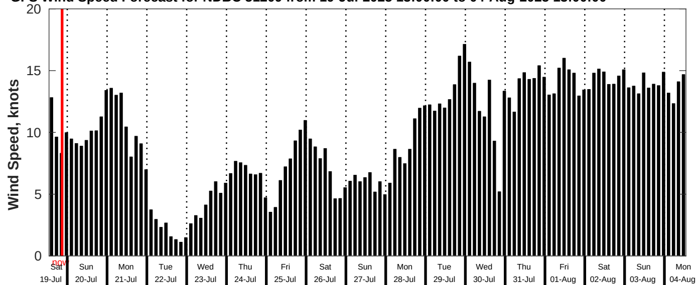
GFS Wind Speed Forecast for NDBC 51209 from 19-Jul-2025 13:00:00 to 04-Aug-2025 13:00:00
