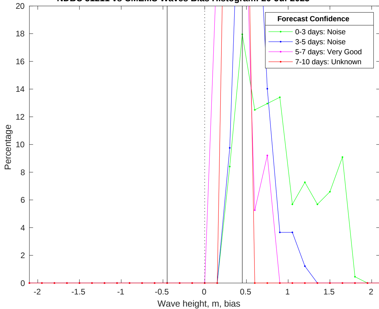
NDBC 51211 vs CMEMS Waves Bias Histogram: 20-Jul-2025
