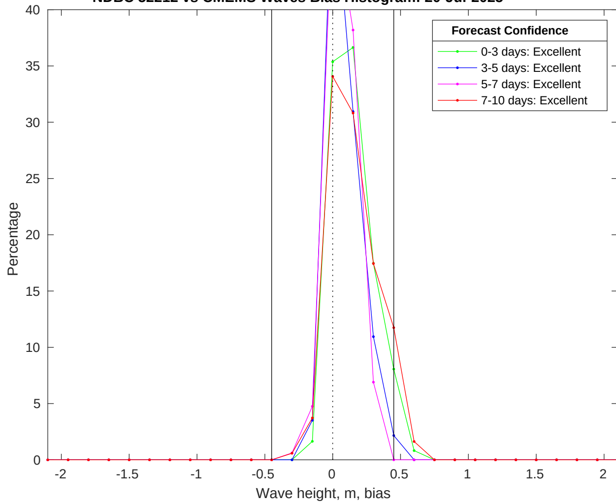
NDBC 52212 vs CMEMS Waves Bias Histogram: 20-Jul-2025
