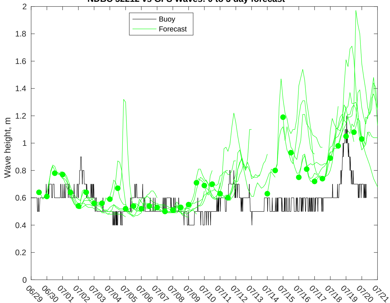
NDBC 52212 vs GFS Waves: 0 to 3 day forecast
