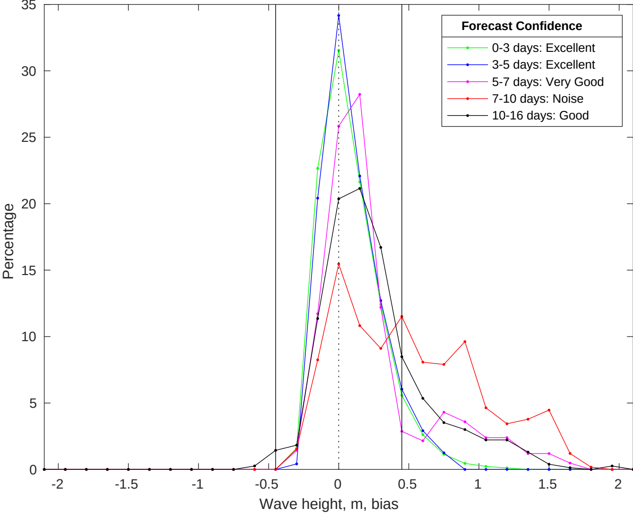
NDBC 52212 vs GFS Waves Bias Histogram: 20-Jul-2025
