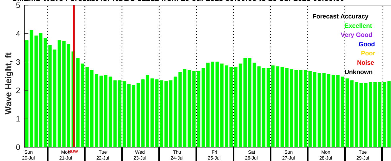
CMEMS Wave Forecast for NDBC 52212 from 19-Jul-2025 09:00:00 to 29-Jul-2025 09:00:00
