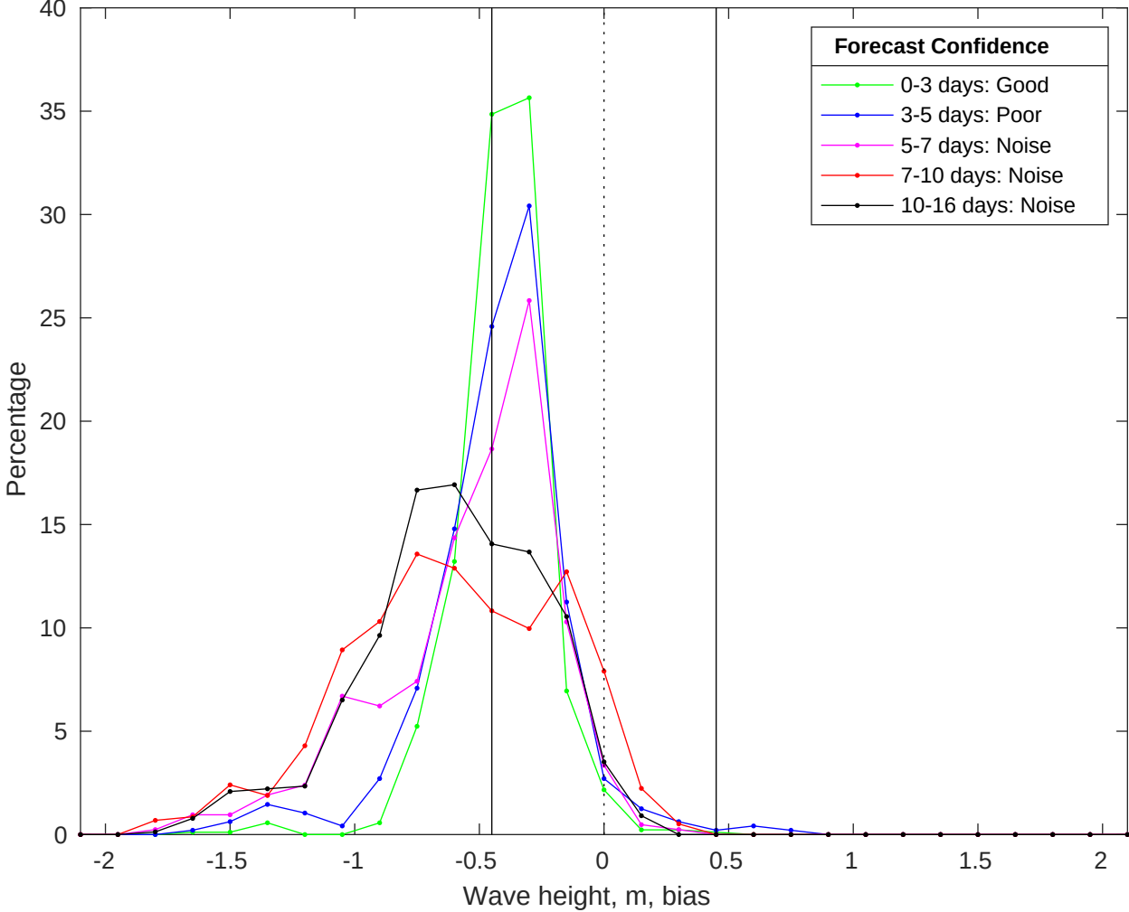
NDBC 52213 vs GFS Waves Bias Histogram: 20-Jul-2025
