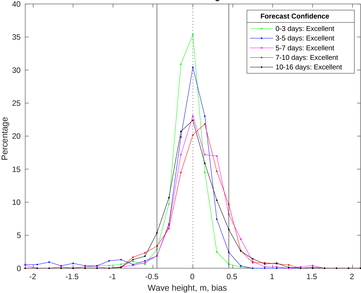
NDBC 41004 vs GFS Waves Bias Histogram: 21-Jul-2025
