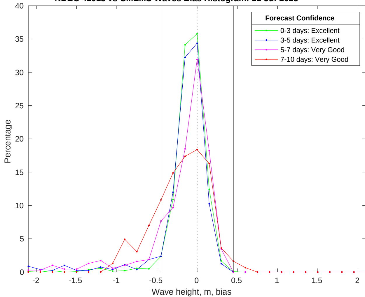
NDBC 41013 vs CMEMS Waves Bias Histogram: 21-Jul-2025
