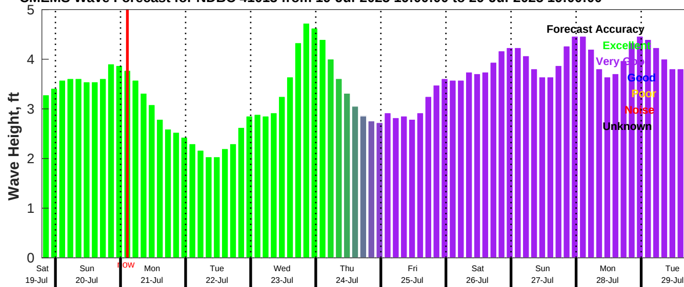
CMEMS Wave Forecast for NDBC 41013 from 19-Jul-2025 19:00:00 to 29-Jul-2025 19:00:00
