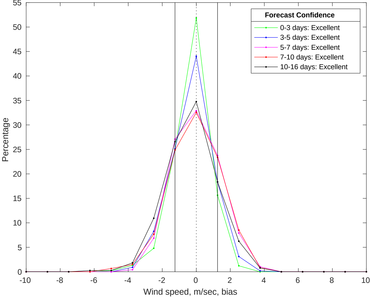
NDBC 41040 vs GFS Winds Bias Histogram: 21-Jul-2025
