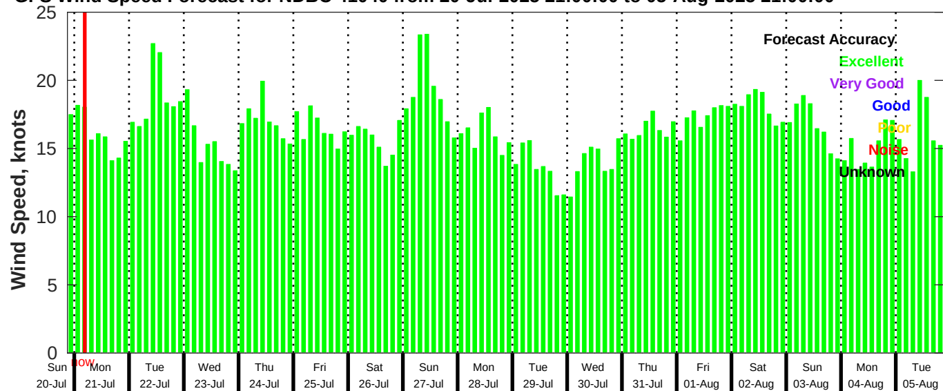
GFS Wind Speed Forecast for NDBC 41040 from 20-Jul-2025 21:00:00 to 05-Aug-2025 21:00:00
