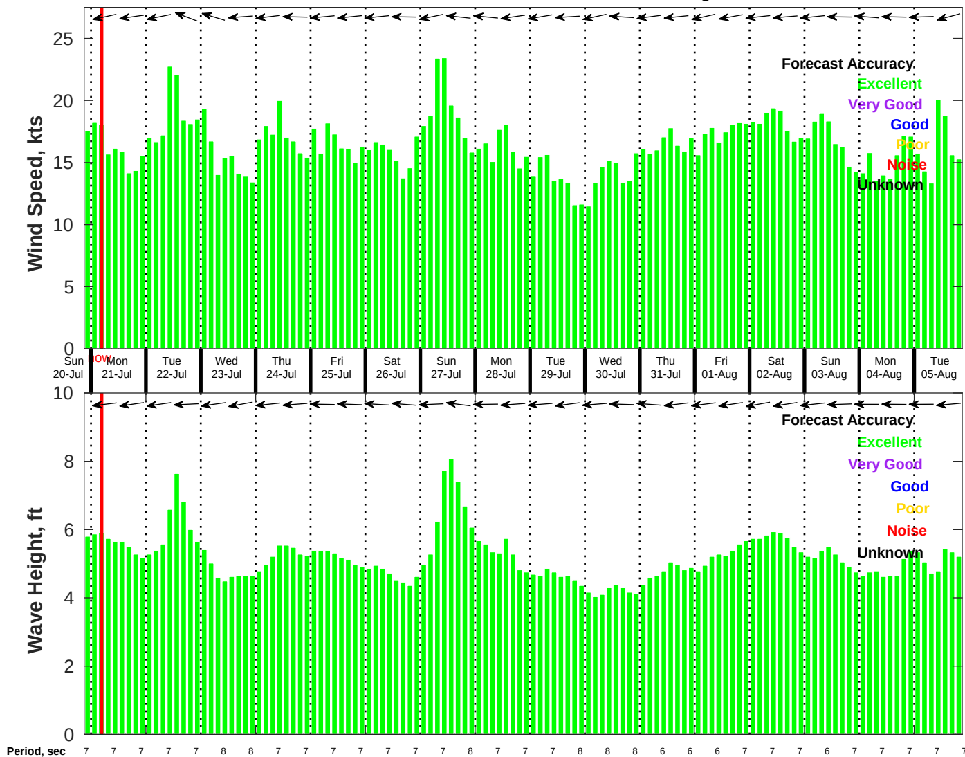
Wind & Wave Forecast for NDBC 41040 from 20-Jul-2025 21:00:00 to 05-Aug-2025 21:00:00
