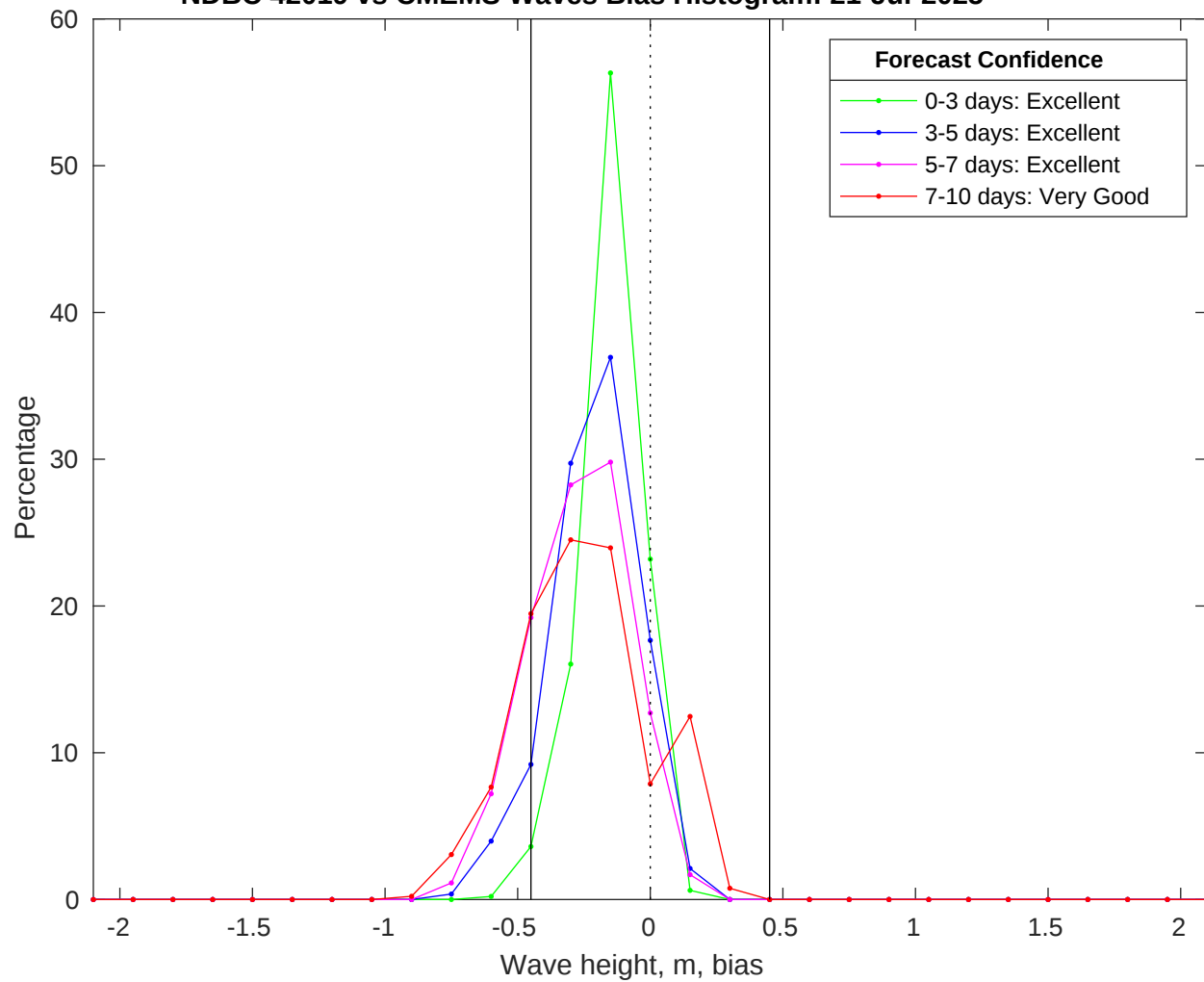
NDBC 42019 vs CMEMS Waves Bias Histogram: 21-Jul-2025
