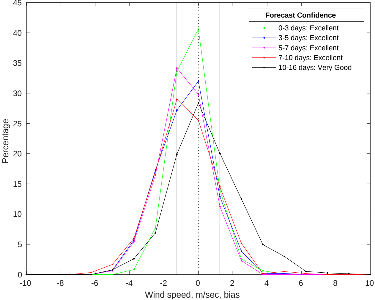
NDBC 42019 vs GFS Winds Bias Histogram: 21-Jul-2025
