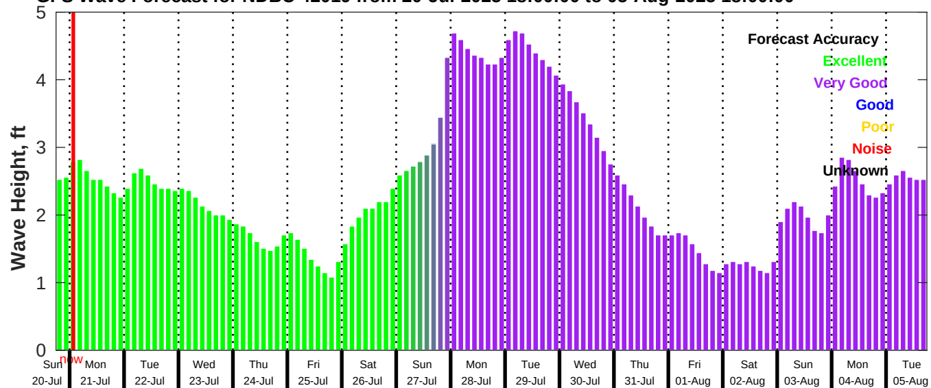
GFS Wave Forecast for NDBC 42019 from 20-Jul-2025 18:00:00 to 05-Aug-2025 18:00:00
