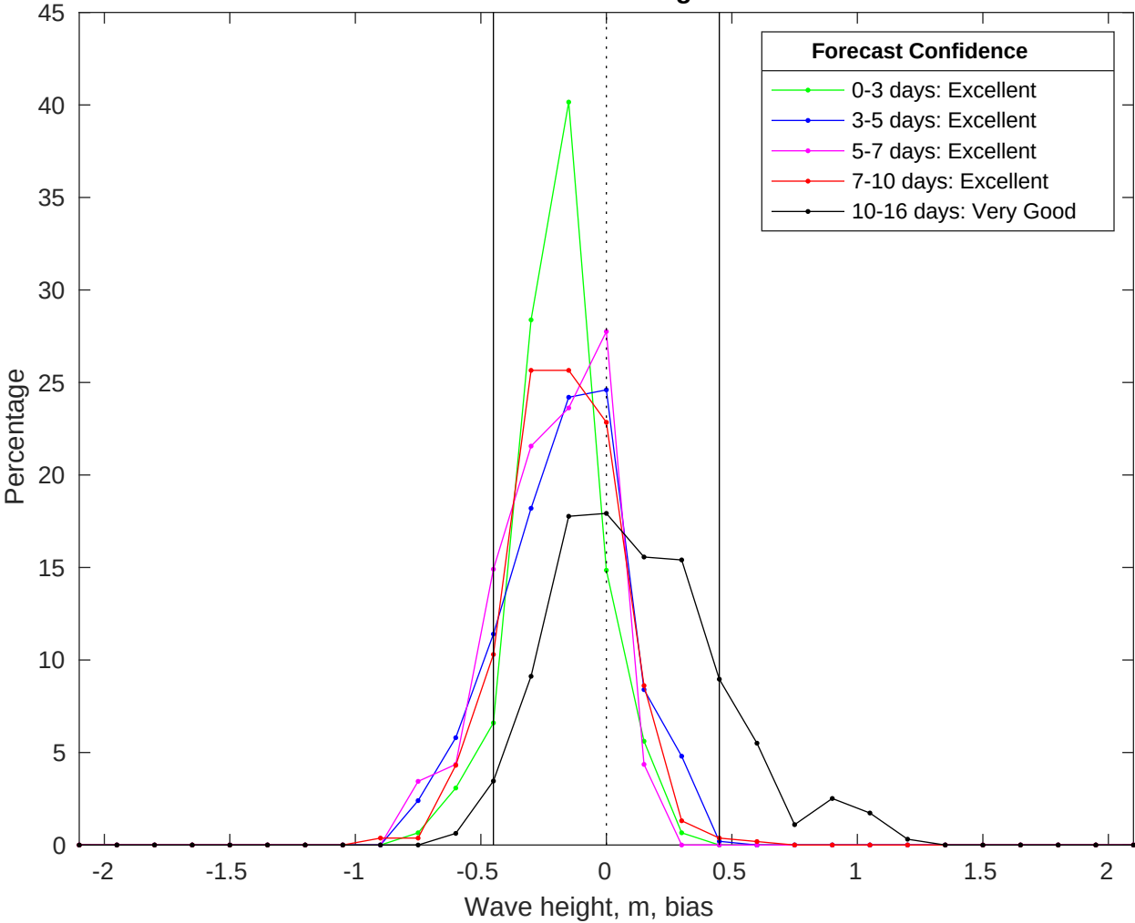
NDBC 42020 vs GFS Waves Bias Histogram: 19-Jul-2025
