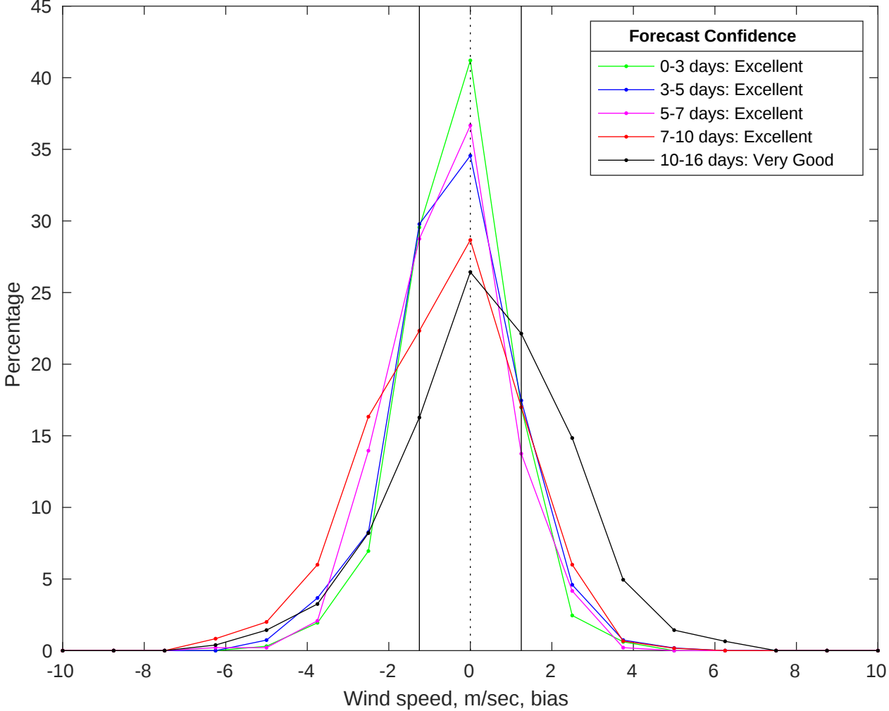
NDBC 42020 vs GFS Winds Bias Histogram: 21-Jul-2025
