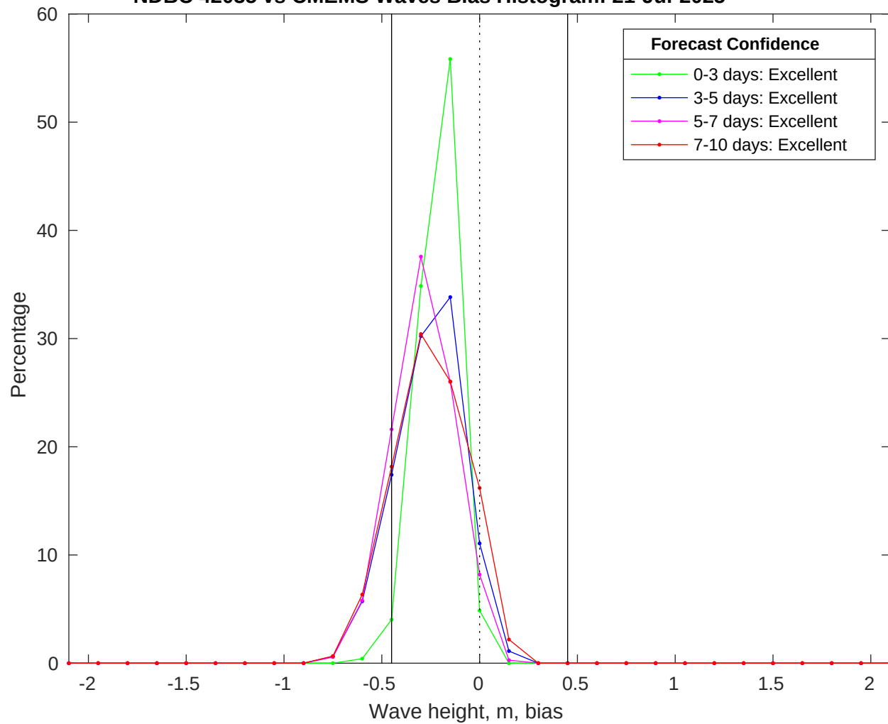
NDBC 42035 vs CMEMS Waves Bias Histogram: 21-Jul-2025
