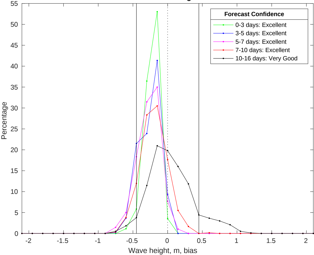
NDBC 42035 vs GFS Waves Bias Histogram: 21-Jul-2025
