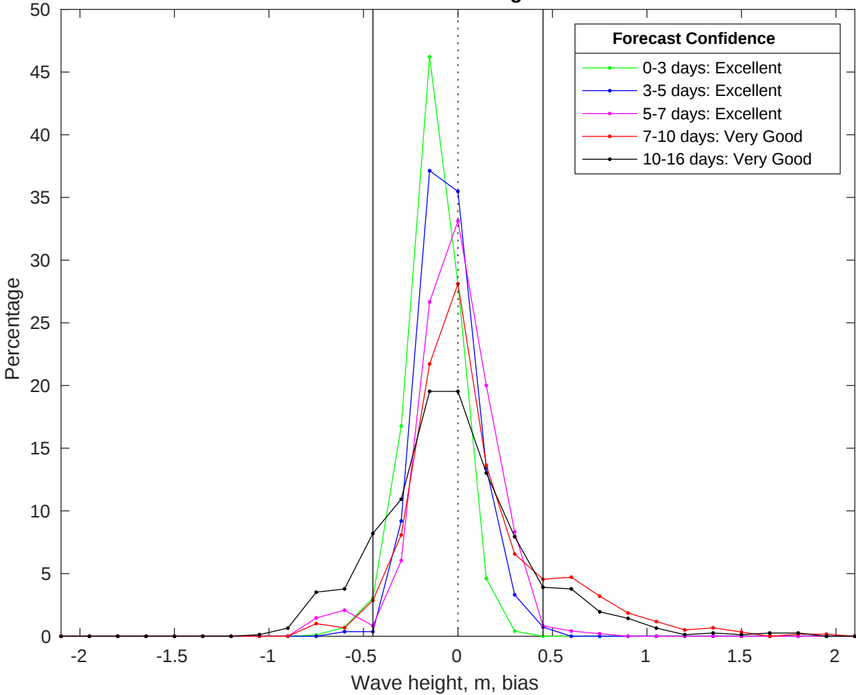
NDBC 42036 vs GFS Waves Bias Histogram: 21-Jul-2025
