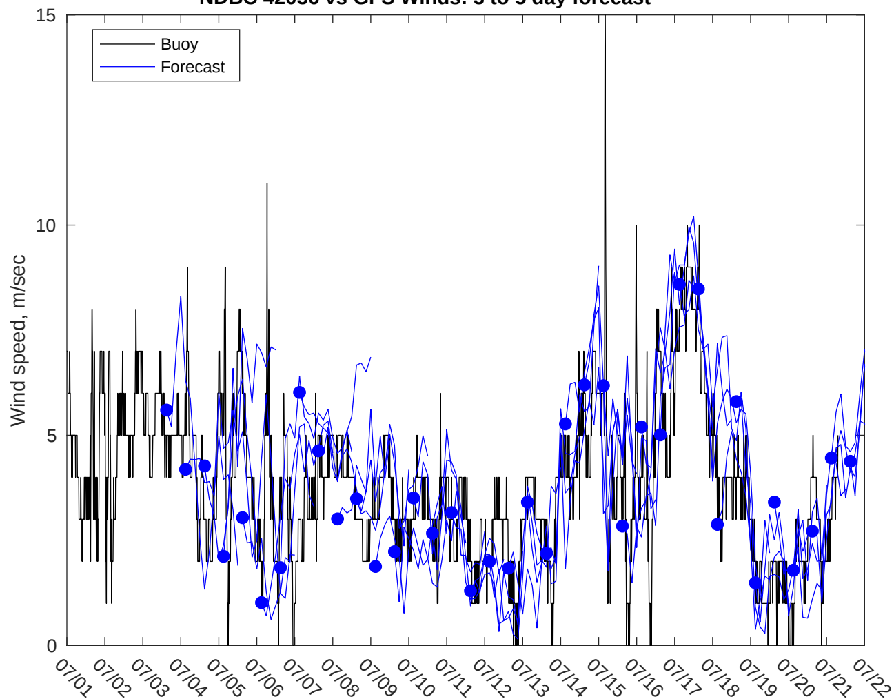
NDBC 42036 vs GFS Winds: 3 to 5 day forecast
