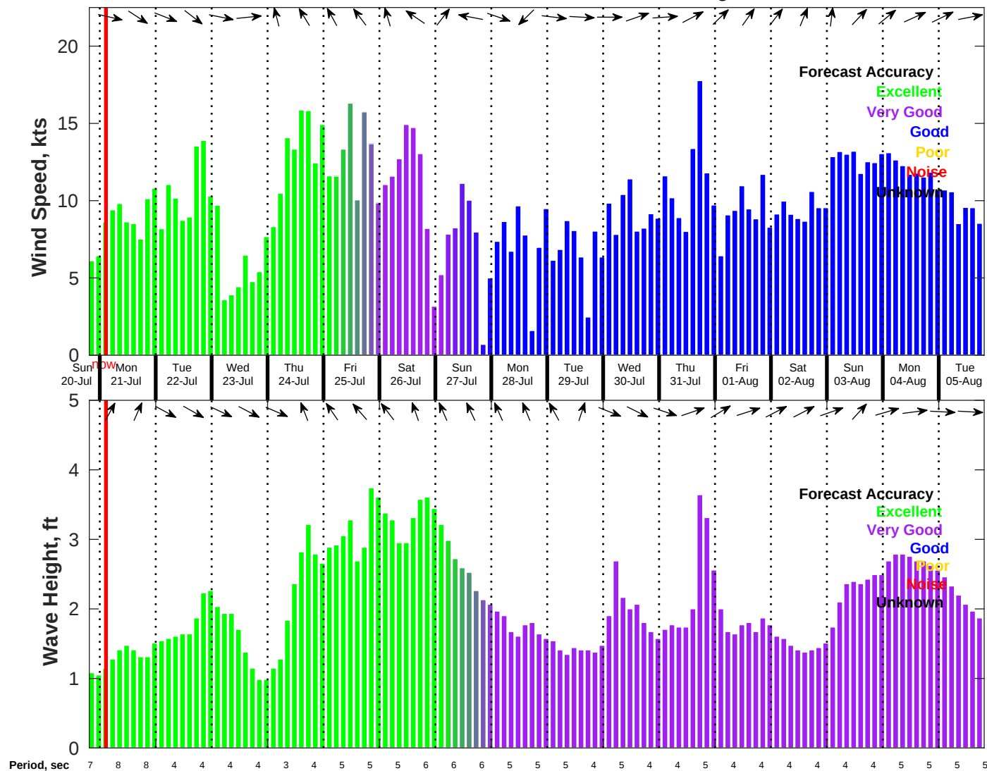
Wind & Wave Forecast for NDBC 42036 from 20-Jul-2025 19:00:00 to 05-Aug-2025 19:00:00
