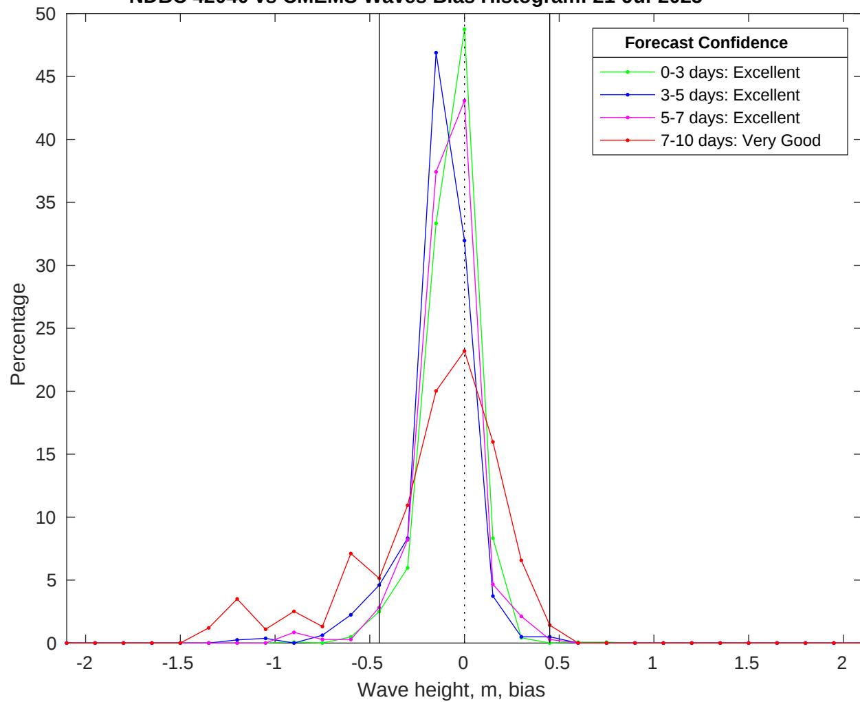
NDBC 42040 vs CMEMS Waves Bias Histogram: 21-Jul-2025
