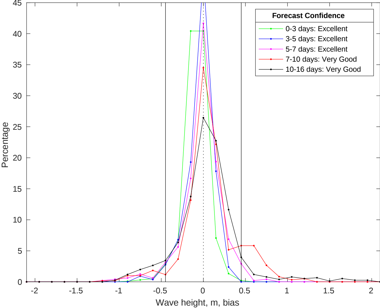
NDBC 42040 vs GFS Waves Bias Histogram: 21-Jul-2025
